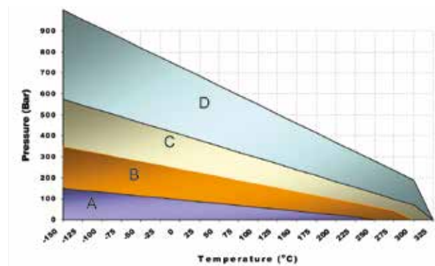
Figure 1, Temperature/Pressure Chart
